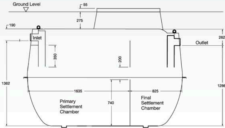
Fortis 12 Septic Tank
