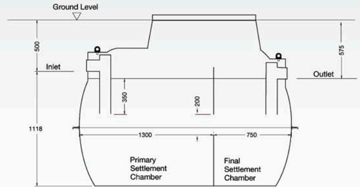
Fortis 5 Septic Tank
