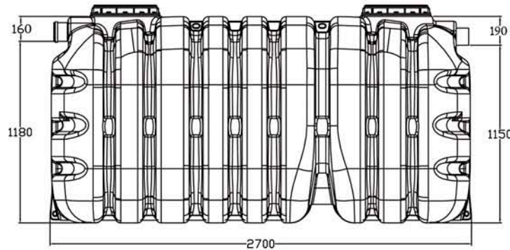
Vento 6 Septic Tank
