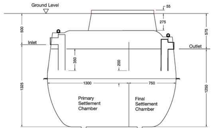
Fortis 6 Septic Tank
